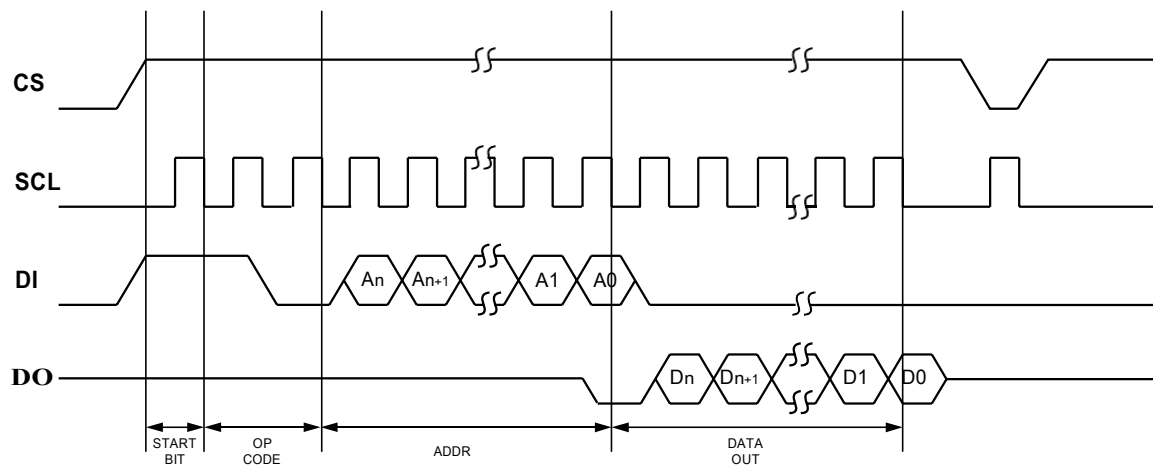
READ Timing
