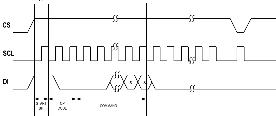
EWEN Timing
