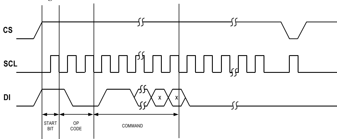
EWEN Timing
