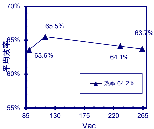
FT8410 (5V-150mA)
