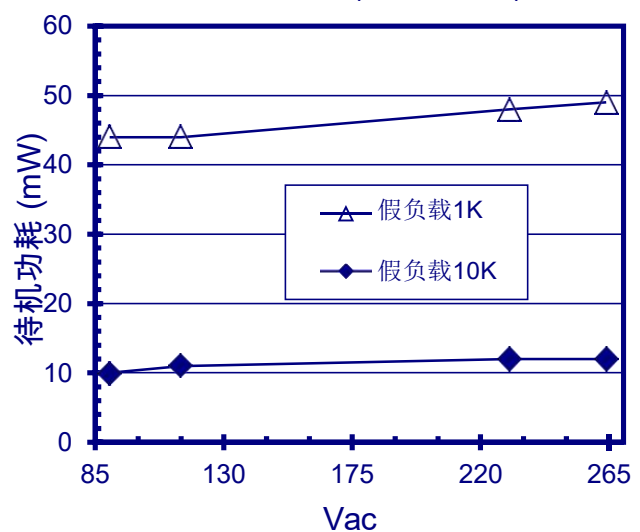
FT8410 (5V-150mA)
