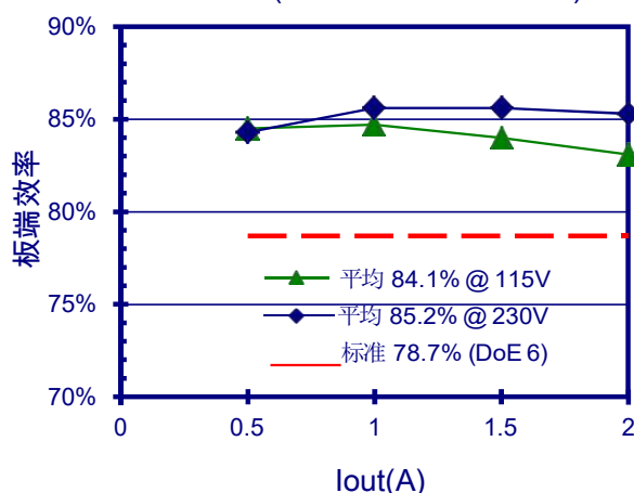
5V-2.0A (FT839ND1+FT8370B)
