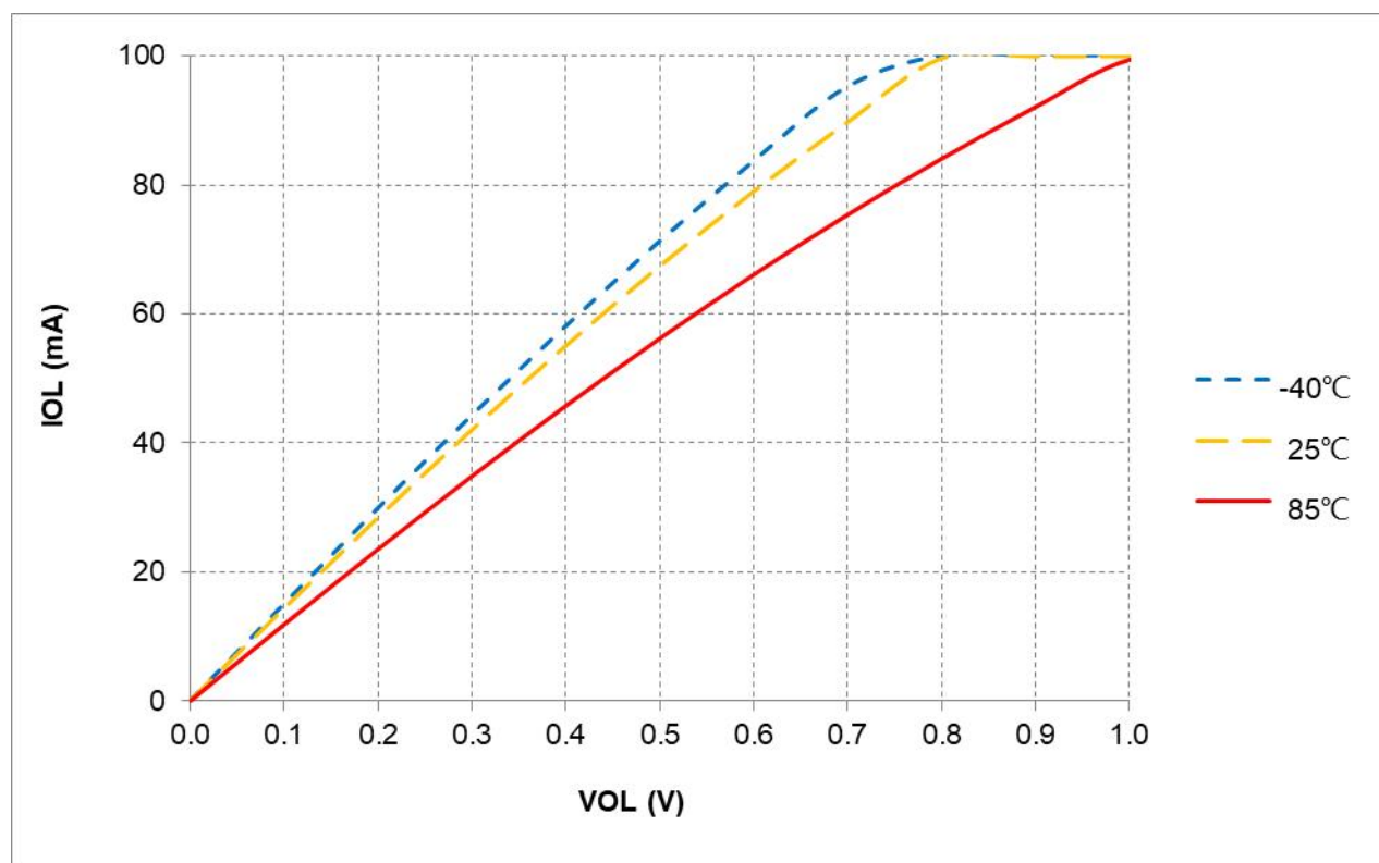
图 17-10 I_{OL} vs. V_{OL} @L1 = 67mA, V_{DD} = 5V
