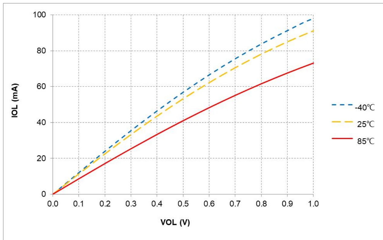
图 17-9 I_{OL} vs. V_{OL} @L0 = 53mA, V_{DD} = 5V
