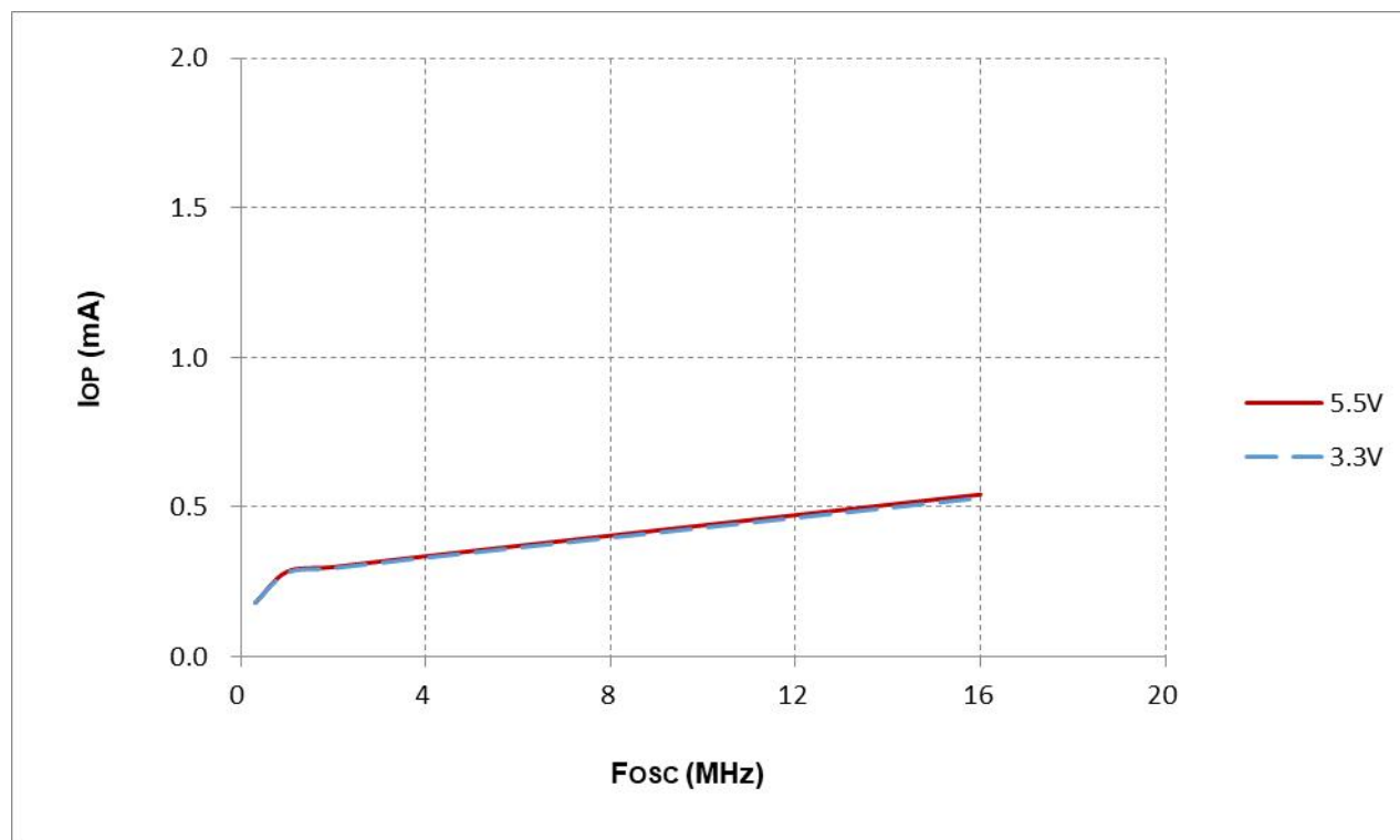
图 17-3 I_{DD} vs. Frequency (4T, T_A = 25^\circ\text{C} )
