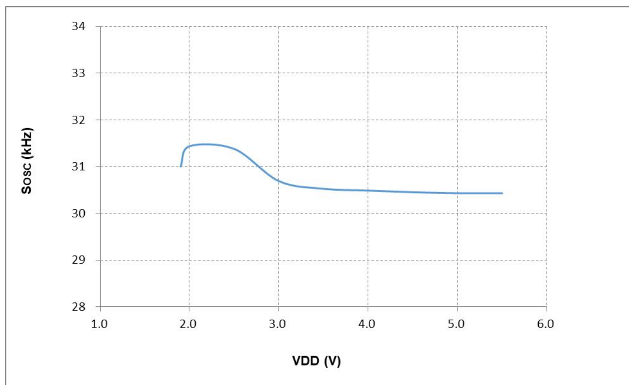
图 17-2 LIRC vs. V_{DD} ( T_A = 25^{\circ}\text{C} )
