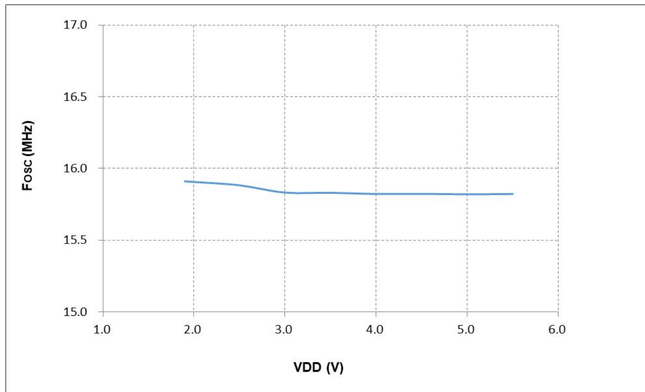
图 17-1 HIRC vs. V_{DD} ( T_A = 25^{\circ}\text{C} )
