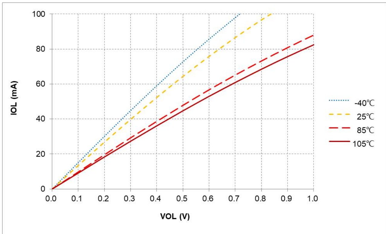
图 3-11 I_{OL} vs. V_{OL} @ L2 = 55\text{mA} , V_{DD} = 5\text{V}
