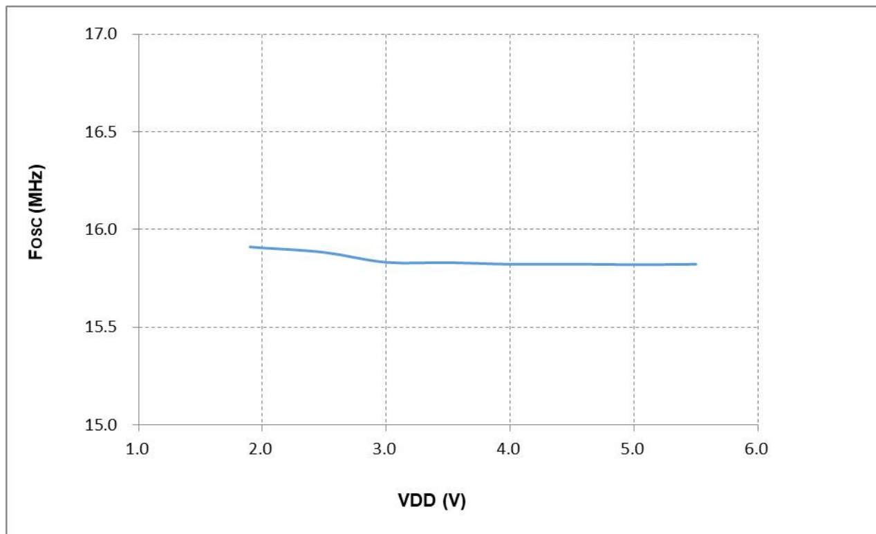
图 16-1 HIRC vs. V_{DD} ( T_A = 25^{\circ}\text{C} )
