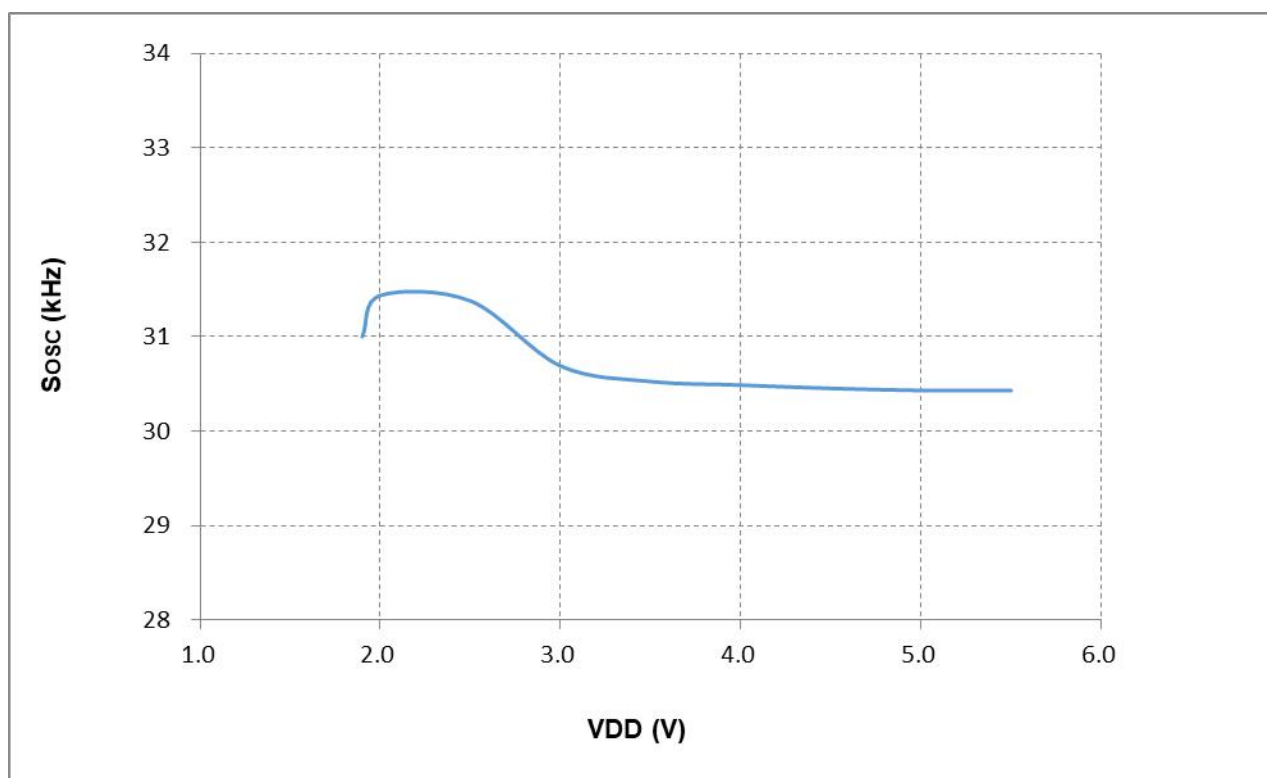
图 16-2 LIRC vs. V_{DD} ( T_A = 25^{\circ}\text{C} )
