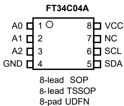
Figure 1: Package types
