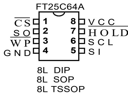
Figure 1: Packaging Types
