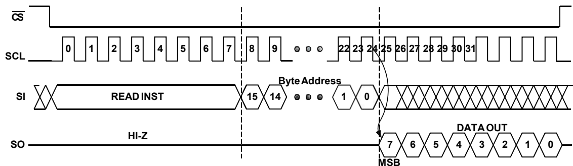
Figure 9: READ Timing
