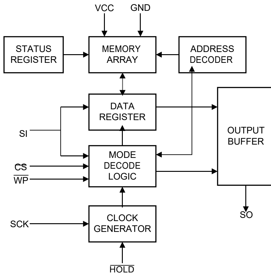
Figure 2: Block Diagram
