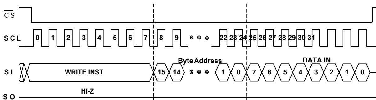
Figure 10: WRITE Timing
