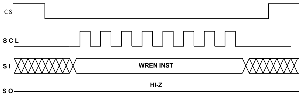
Figure 5: WREN Timing
