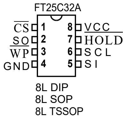
Figure 1: Packaging Types
