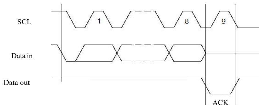
Figure 2: Timing diagram for output ACKNOWLEDGE
