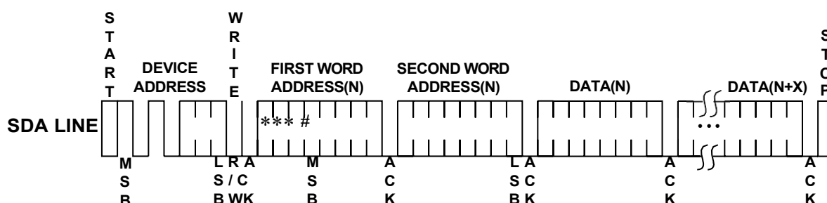
Figure 4: Page Write
