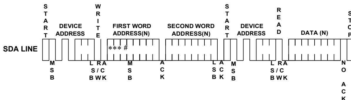
Figure 7: Random Read
