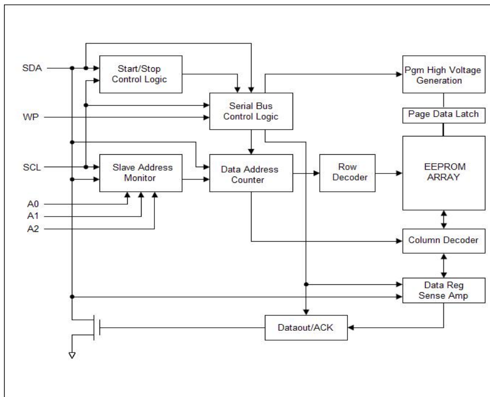
Figure 2: Block Diagram
