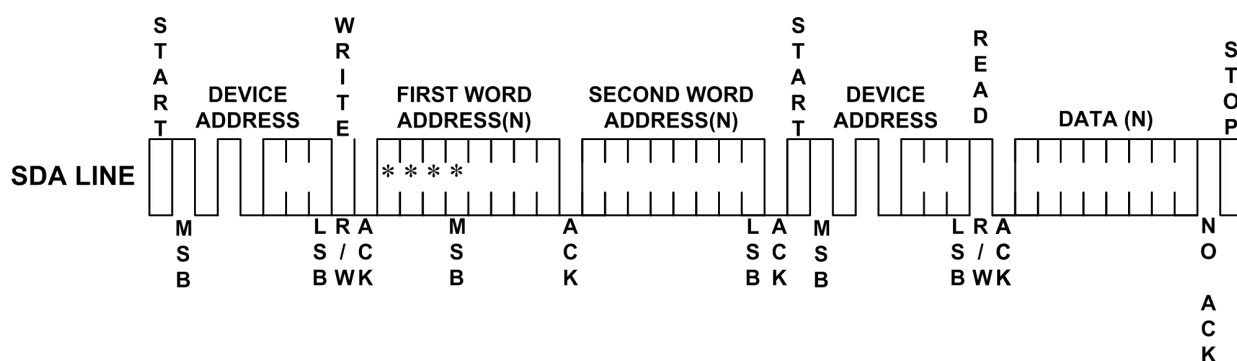
Figure 7: Random Read
