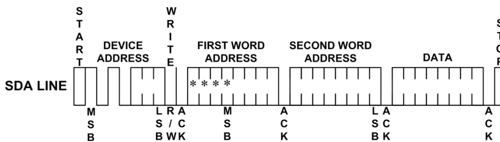
Figure 3: Byte Write
