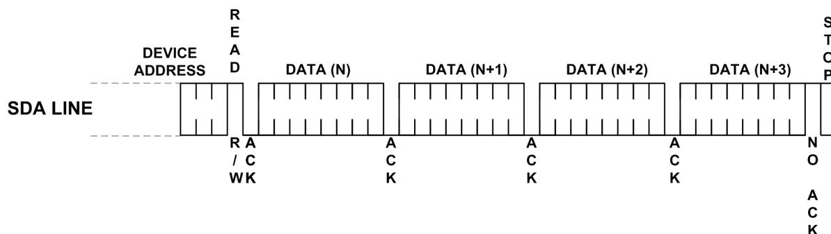
Figure 6: Sequential Read
