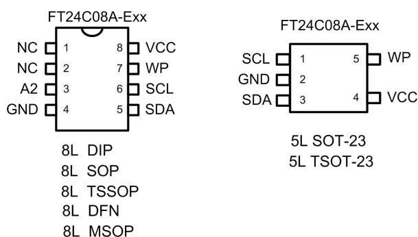
Figure 1: Package types
