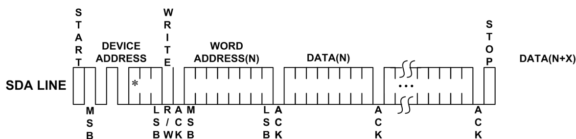
Figure 6: Page Write
