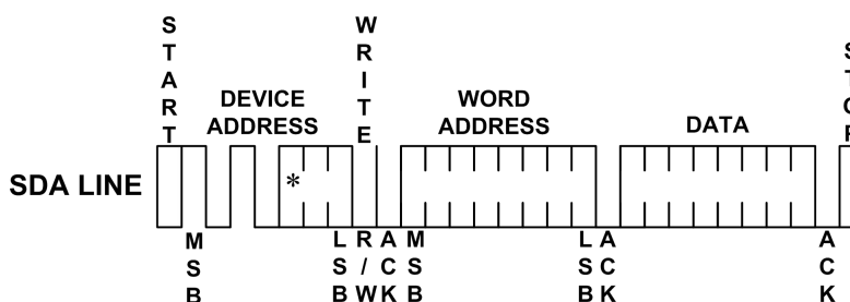
Figure 5: Byte Write
