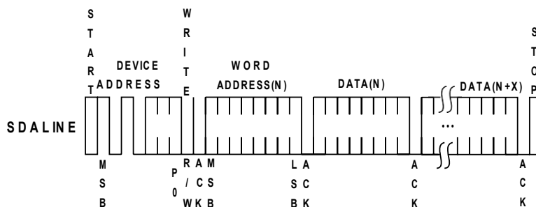
Figure 6: Page Write
