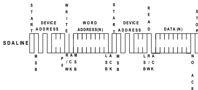
Figure 9: Random Read
