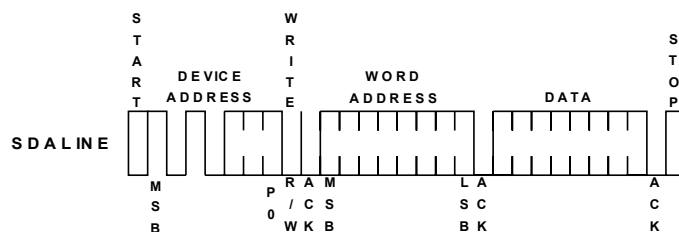
Figure 5: Byte Write
