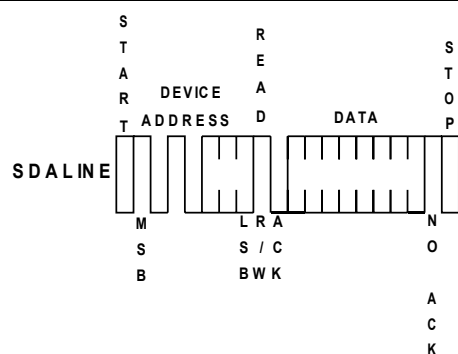
Figure 7: Current Address Read
