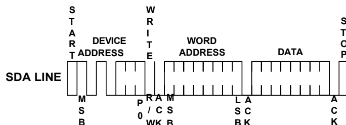
Figure 5: Byte Write
