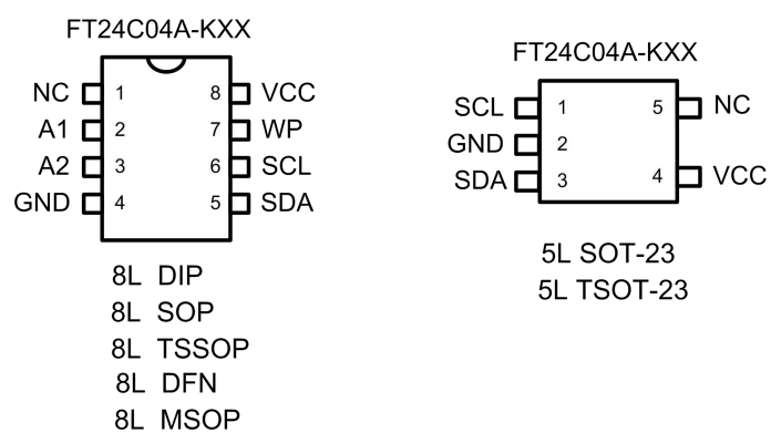
Figure 1: Package types
